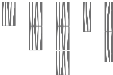
Above left: Silvus24 exterior/interior sconce in 1, 2, and 3-unit high configurations. Above right: Silvus30 interior/exterior
